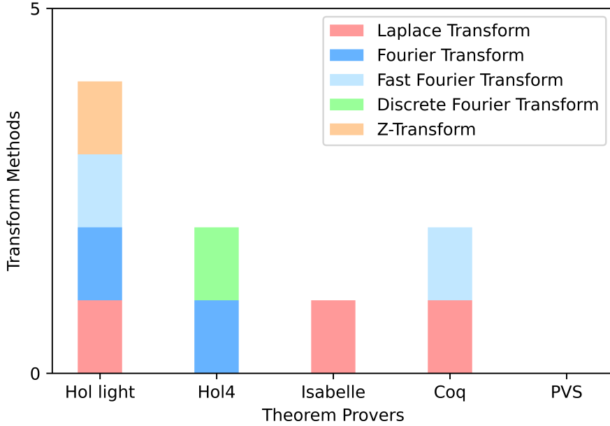
Figure 2: Support for Transform Methods in Higher-order-logic Theorem Provers
