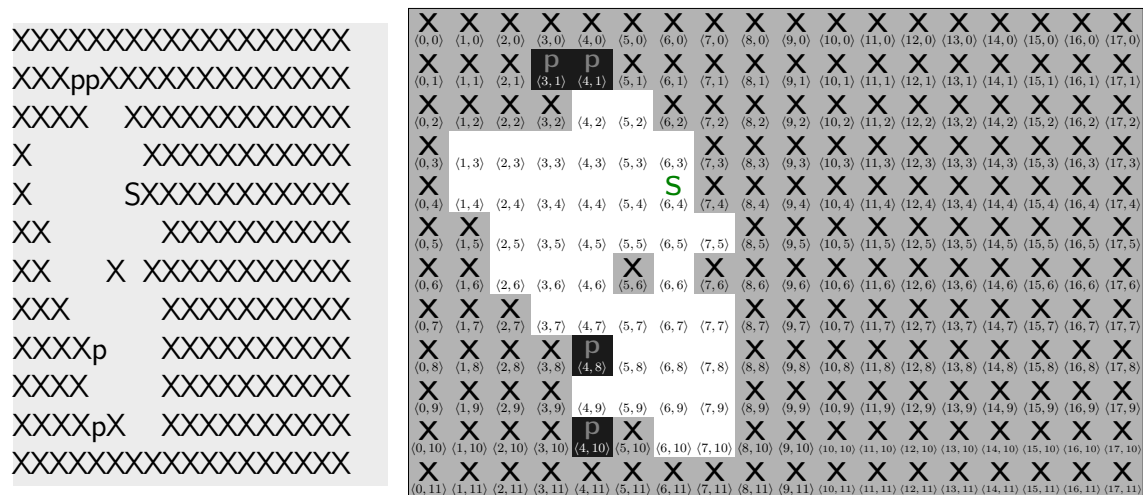
Figure 1: An example map of the Wumpus cave with the starting position marked at \langle 6, 4 \rangle . and several pits marked with ps. The text representation (left) is used in the problem files.
