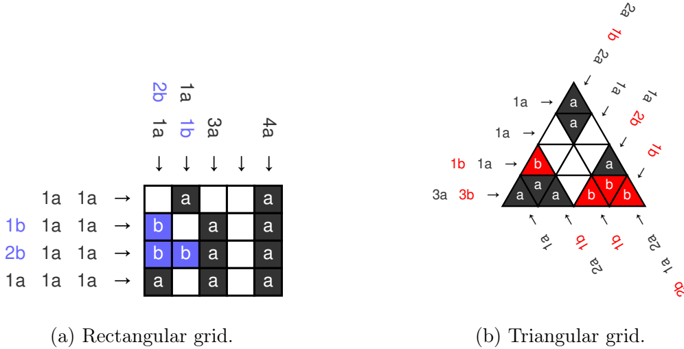
Figure 1: Two example generalized nonograms (solved).
