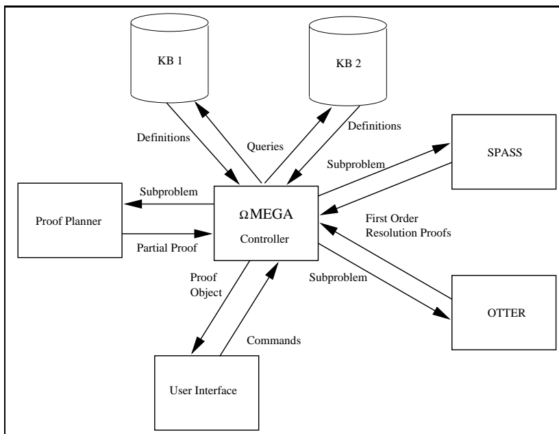
Figure 1: Distributed Mathematical Services in \Omega MEGA
