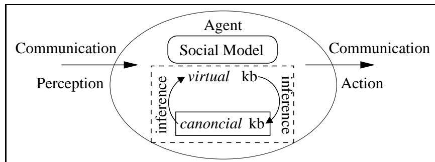
Figure 2: A (Social) Agent Architecture
