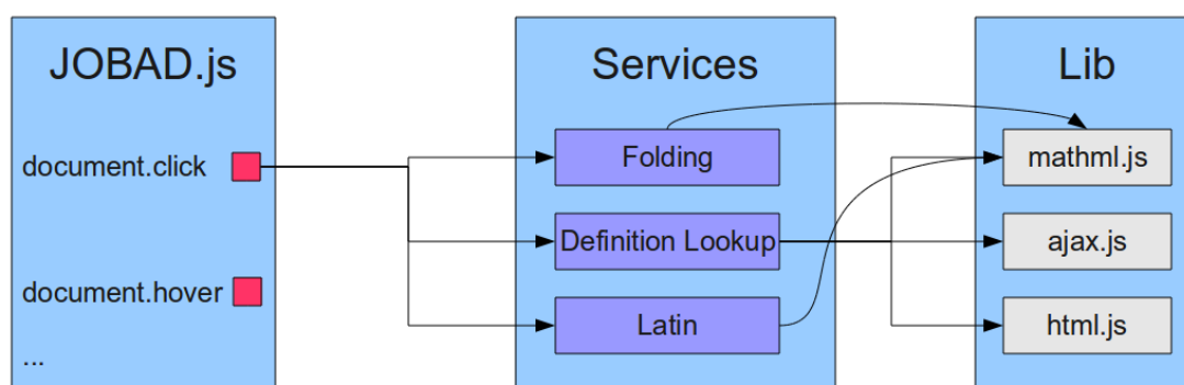
FIGURE 2.1: JOBAD internal architecture
