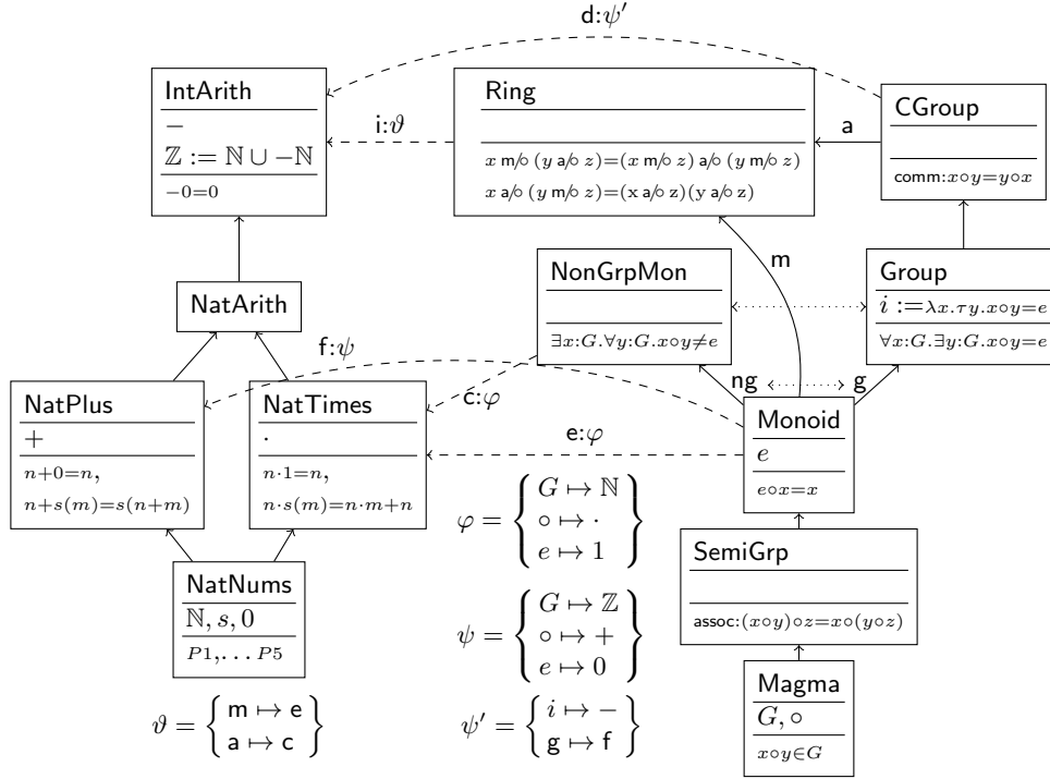
Fig. 1. A MMT Graph for Elementary Algebra
