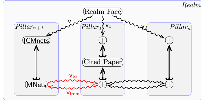
Fig. 6. Aggregation graph for equivalence recaps (Example 2)
