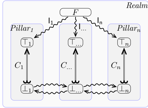
Fig. 1. The architecture of a realm
