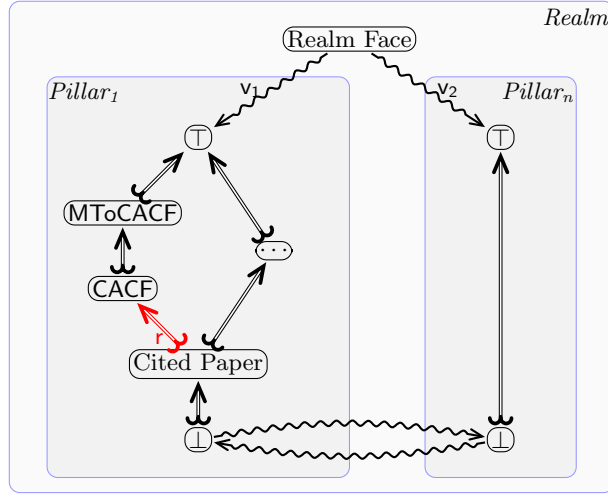
Fig. 4. Aggregation graph for plain recaps (Example 1)
