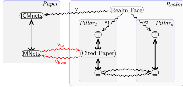
Fig. 5. Publication graph for equivalence recaps (Example 2)
