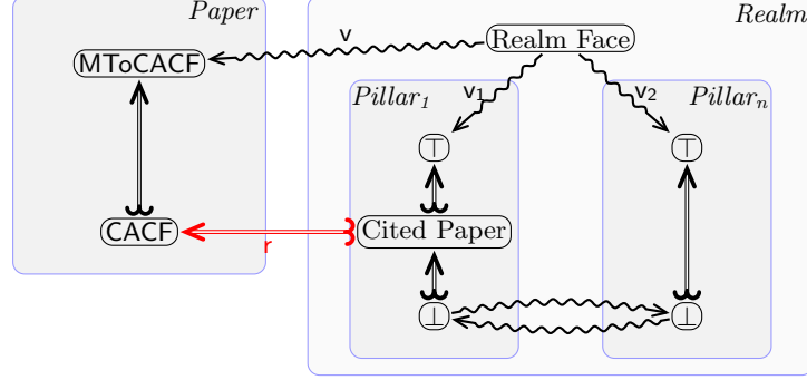
Fig. 3. Publication graph for plain recaps (Example 1)
