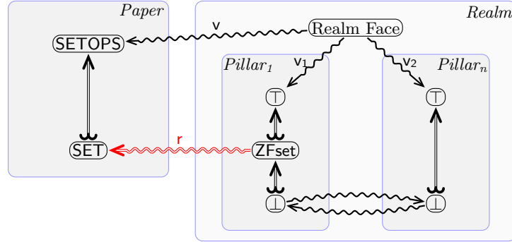
Fig. 8. Publication graph for generalization/unspeficd recaps (Example 4)
