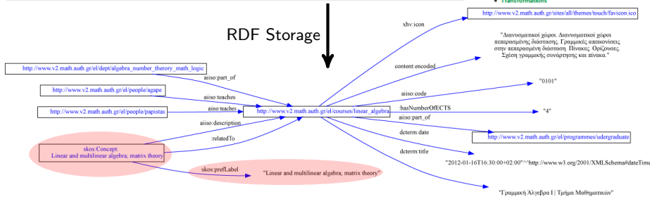
Fig. 1. Annotating the scientific fields of a course on the new AUTH School of Mathematics site, using MSC/SKOS and Drupal 7 semantic mappings (cf. [6])
